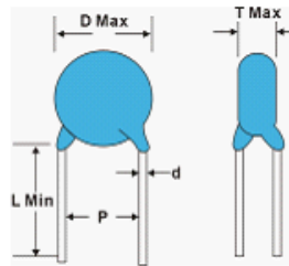
Capacitors with 7.5 mm (0.30") to 15 mm (0.40") lead spacing(P)
